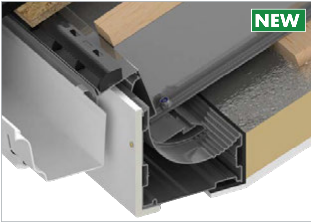
New 15° and 25° fixed pitch options allow for simpler roof designs (Variable 5°-35° pitch shown)
